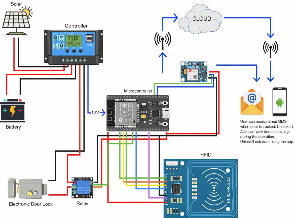
Figure 2. System Architecture of the Solar-Powered RFID and IoT-Based Automatic Door Locking System
